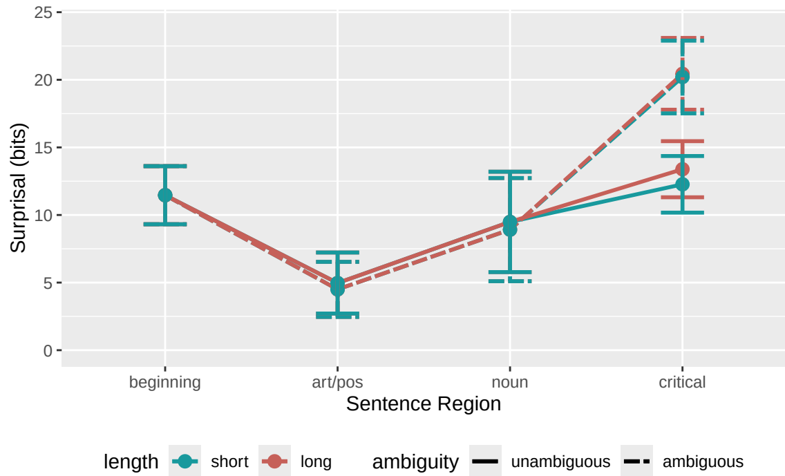
LLM Surprisal by Sentence Region (final items)
