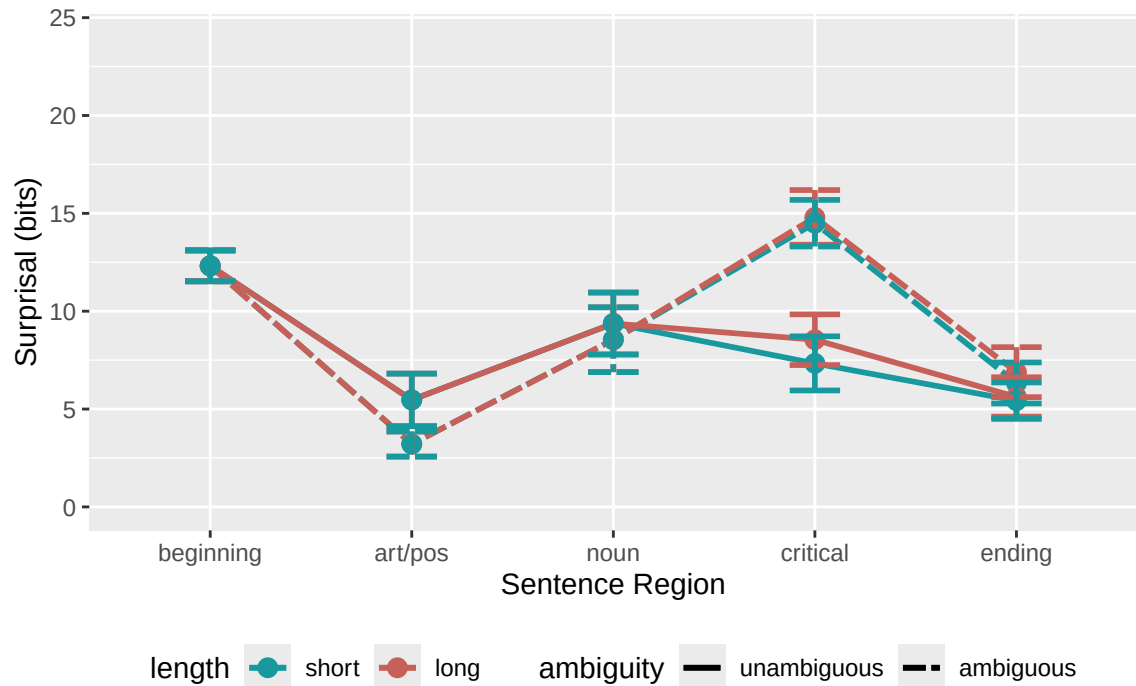
LLM Surprisal by Sentence Region (nonfinal items)
