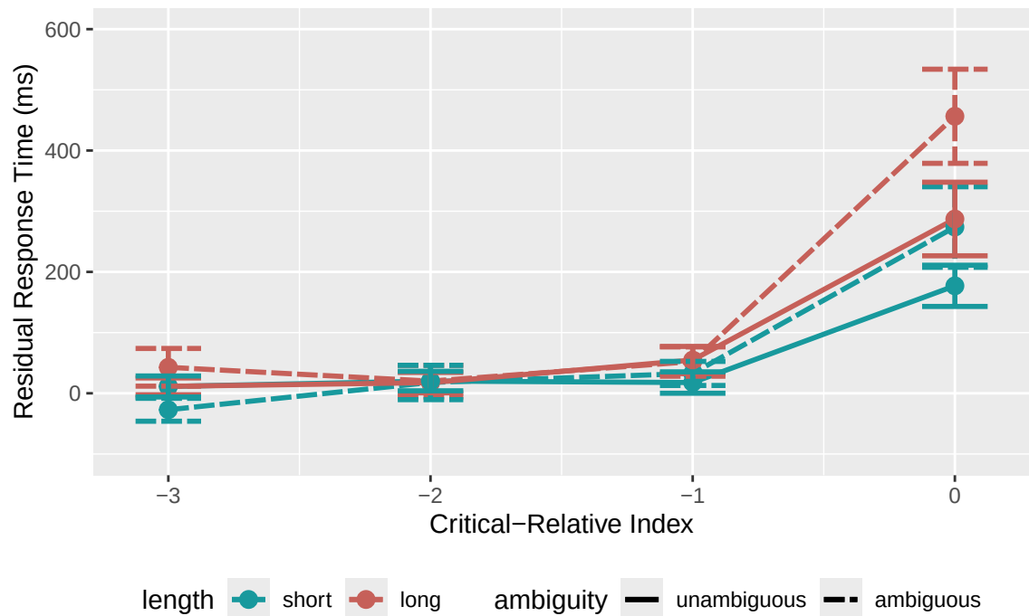
Residual RTs by Critical-Relative Index (final conditions)
