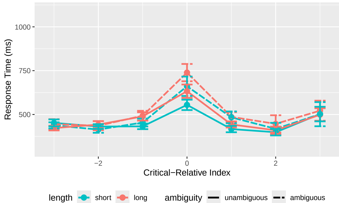
Empirical RTs by Critical-Relative Index ( all conditions)
