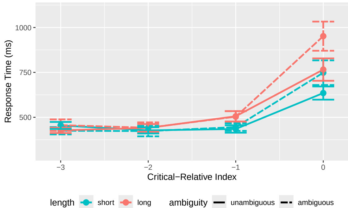
Empirical RTs by Critical-Relative Index ( final conditions)
