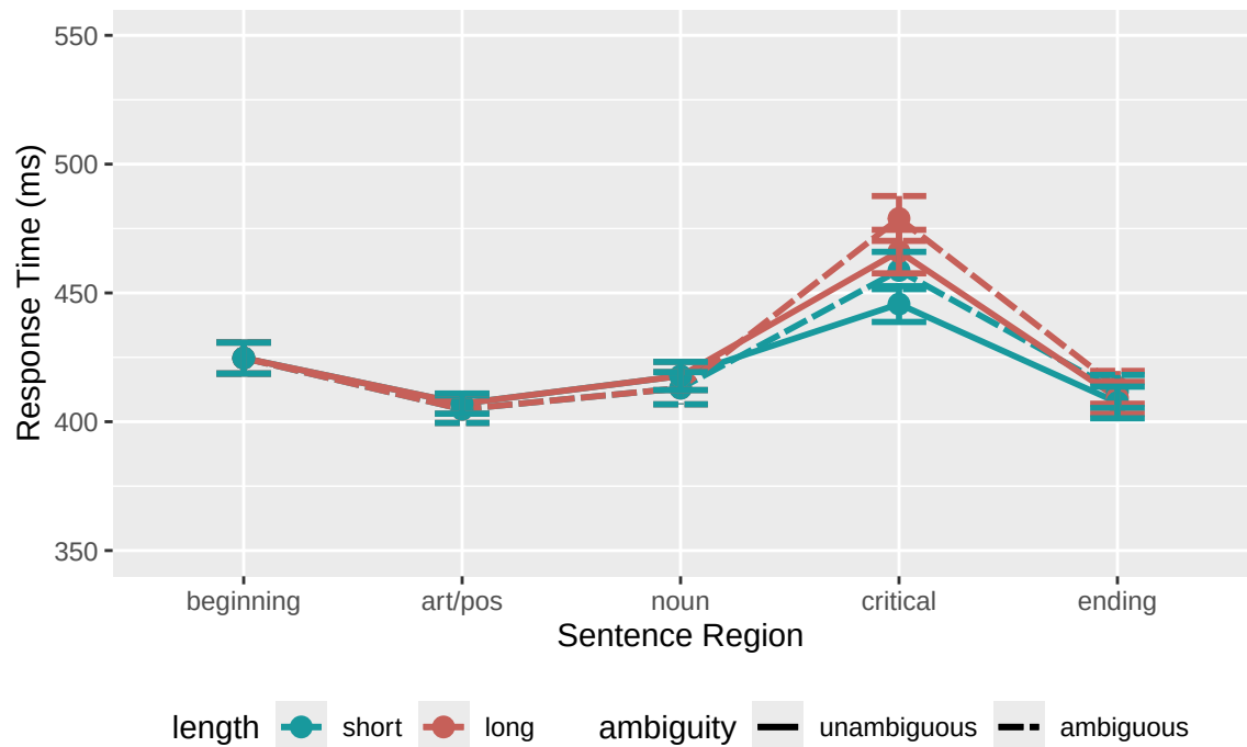
Predicted RTs by Sentence Region (nonfinal conditions)
