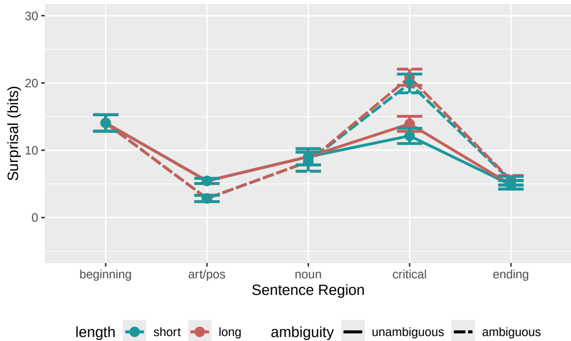
LLM Surprisal by Sentence Region (all conditions)
