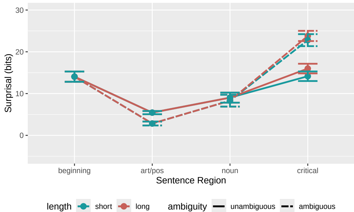
LLM Surprisal by Sentence Region (final conditions)
