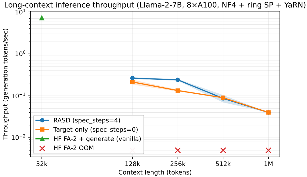
Figure 4: Throughput vs. context length. RASD spec mode (●) and matched target-only baseline (■) at 4 contexts \times 3 seeds; vanilla HF FA-2 generate() (▲) at 32k only, OOM markers (×) for \geq 128k . Bands are 95% bootstrap CI over 3 seeds. Both axes log scale.
