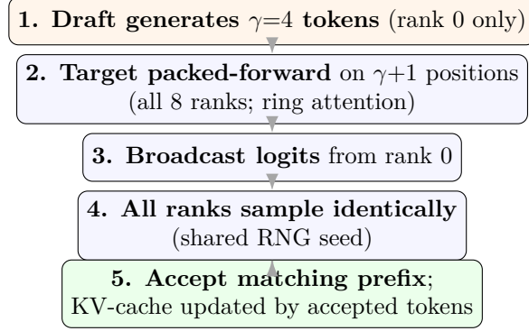
Figure 2: Sequence of one RASD decode round. The draft proposes \gamma=4 tokens on rank 0 (step 1); the target verifies them in a single packed forward over \gamma+1 positions on all 8 ranks via ring attention (step 2); target logits are broadcast from rank 0 (step 3) and every rank samples identically using a shared RNG seed (step 4); the longest matching prefix is accepted and the KV cache is updated by the accepted tokens (step 5) [Leviathan et al., 2023, Chen et al., 2023a]. The 8-rank topology these steps execute on is shown in Fig. 1.
