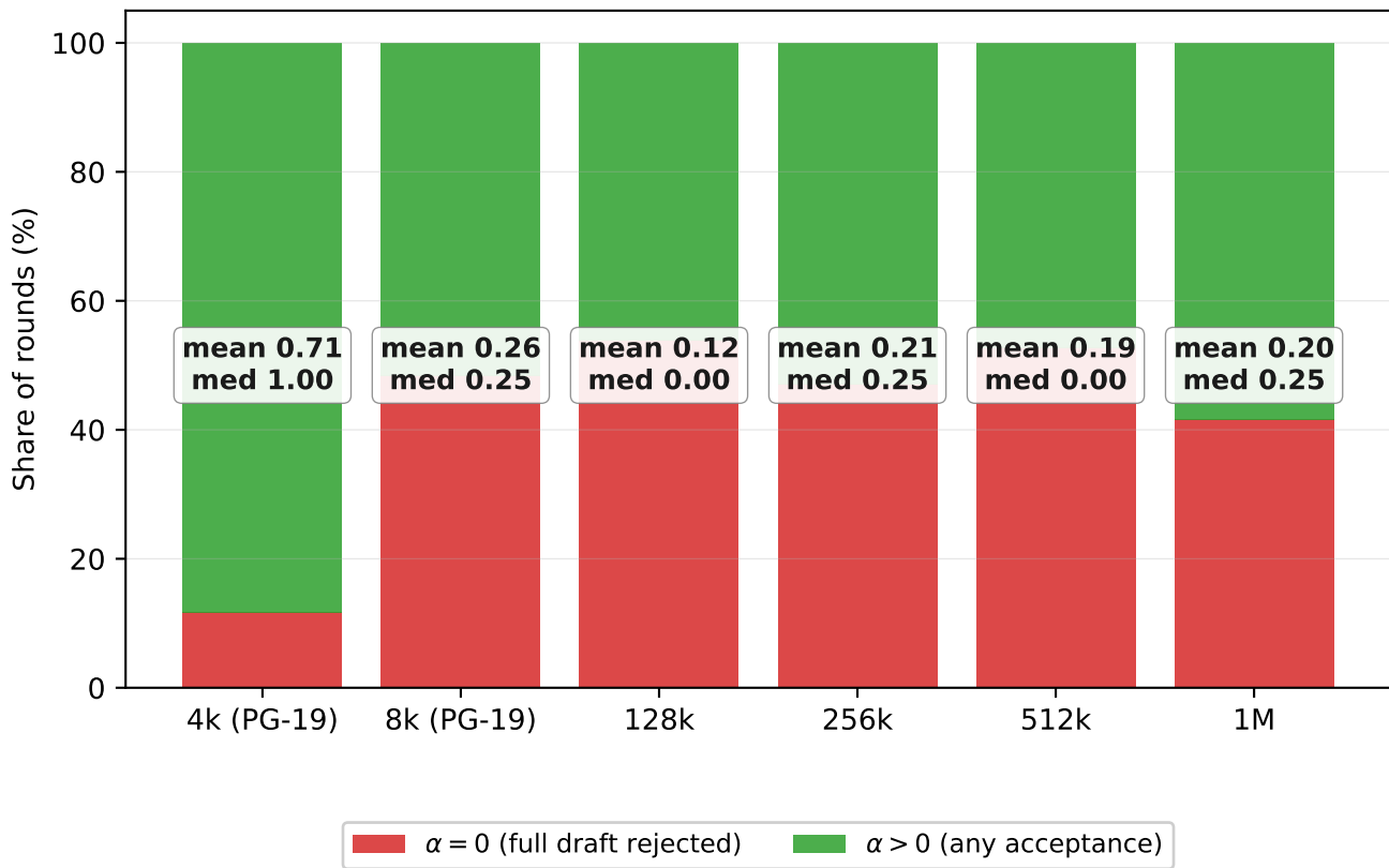
Bimodality of \alpha : full-rejection vs any-acceptance share by context
