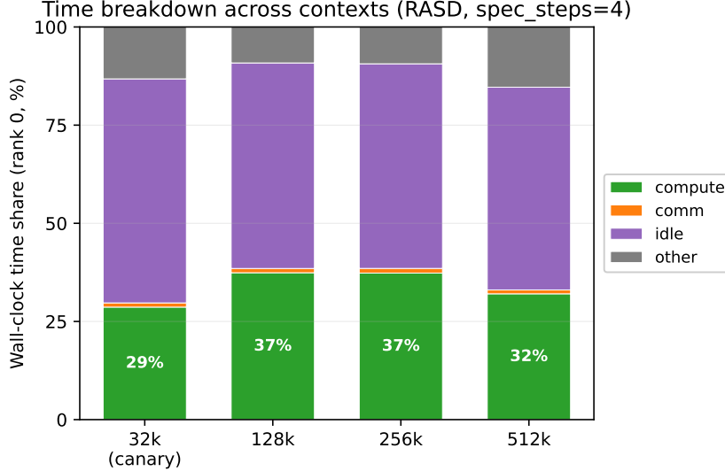
Figure 5: Stacked-bar time breakdown for rank-0 across contexts. “Compute” is real GPU work (matmul, attention, layernorm, etc.); “comm” is NCCL + ring-exchange collectives; “idle” is wall not attributable to GPU events (rank-0 waiting on other ranks); “other” is allocator and kernel-launch overhead. Annotated value is the compute share.
