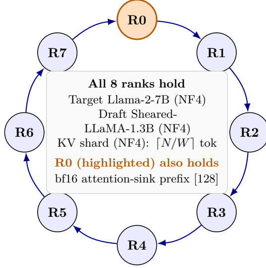
Ring topology of 8 ranks at one decode round
