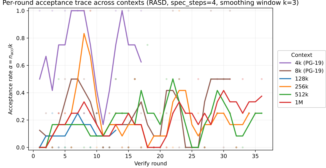
Figure 6: Per-round acceptance \alpha = n_{\text{acc}}/k for RASD across six contexts (4k and 8k with PG-19 prompts, 128k–1 M with synthetic prompts), smoothed by a 3-round rolling mean. Raw points are drawn faded behind the smoothed line. The traces show the per-round texture that the aggregate means in Table 4 hide.
