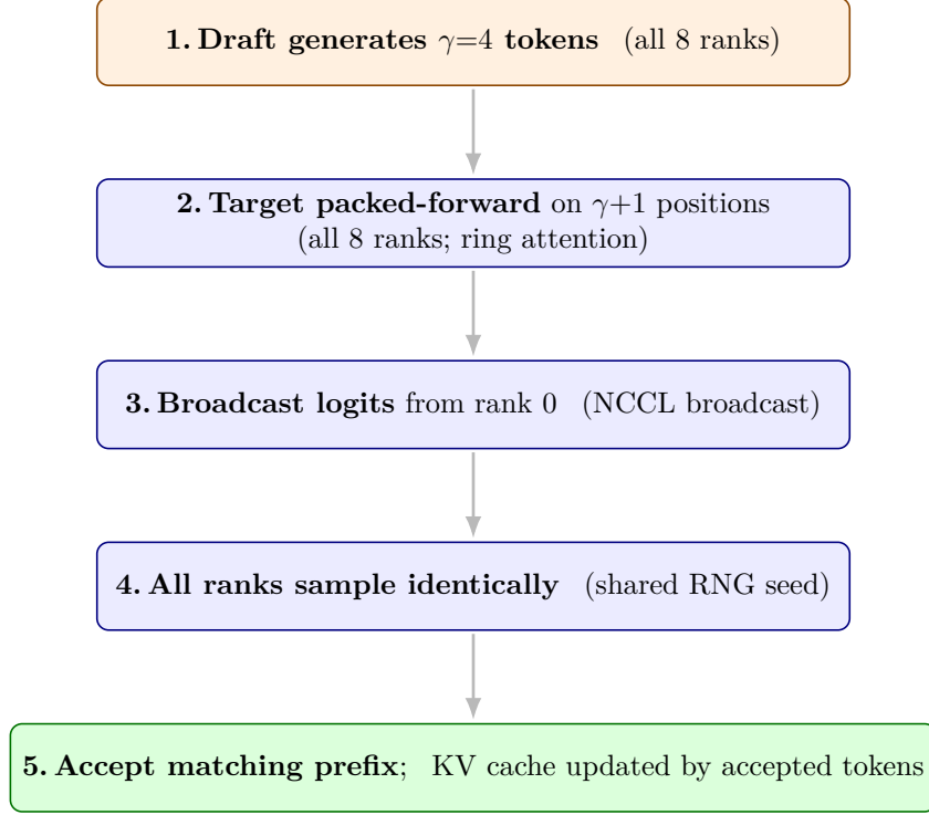
Figure 2: Sequence of one RASD decode round. The draft proposes \gamma=4 tokens on all 8 ranks (step 1); the target verifies them in a single packed forward over \gamma+1 positions on all 8 ranks via ring attention (step 2); the draft and target logits are broadcast from rank 0 (step 3) and every rank samples identically using a shared RNG seed (step 4); the longest matching prefix is accepted and the KV cache is updated by the accepted tokens (step 5) [Leviathan et al., 2023, Chen et al., 2023a]. The 8-rank topology these steps execute on is shown in Fig. 1.
