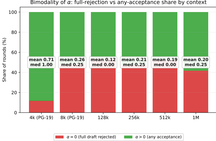
Figure 7: Bimodality view of \alpha : per-context share of verify rounds that fully reject the draft ( \alpha = 0 , red) vs. accept at least one token ( \alpha > 0 , green). Annotations report the per-context mean and median \alpha . At every long context (128k–1M), roughly half of all verify rounds fully reject the draft — the structural signal the per-context means obscure.
