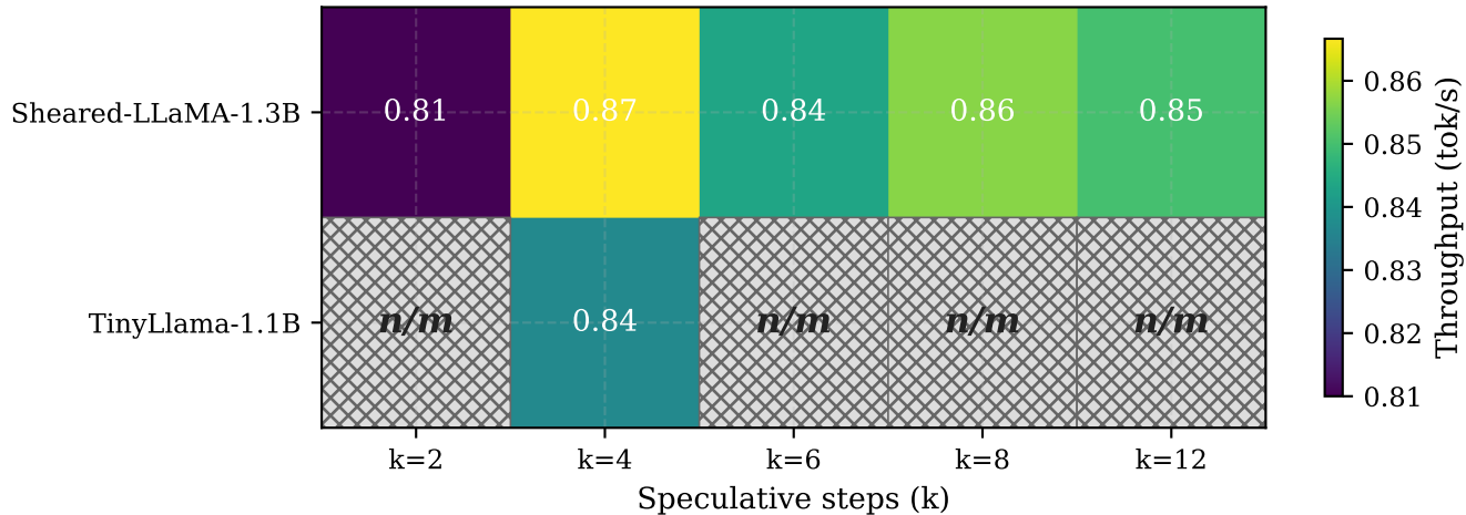
M3 ablation: Throughput (tok/s) (ctx=64k, 8×A100-SXM4-40GB)
