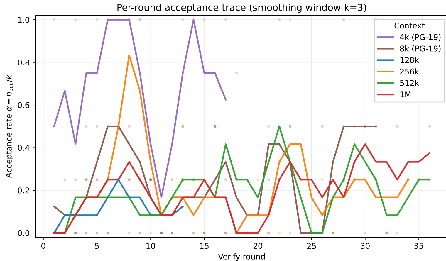
Per-round acceptance rate across contexts (RASD, spec_steps=4)
