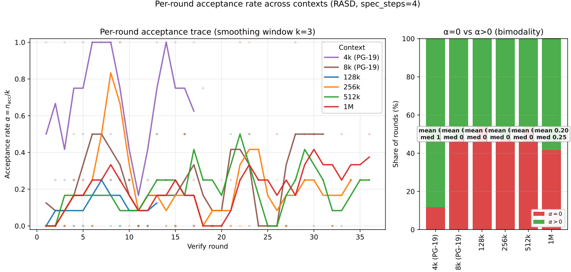
Figure 6: (Left) per-round acceptance \alpha = n_{acc}/k for RASD across six contexts (4k and 8k with PG-19 prompts, 128k–1M with synthetic prompts), smoothed by a 3-round rolling mean. Raw points faded behind. (Right) Bimodality view: share of rounds at \alpha = 0 vs \alpha > 0 per context, annotated with mean and median \alpha .
