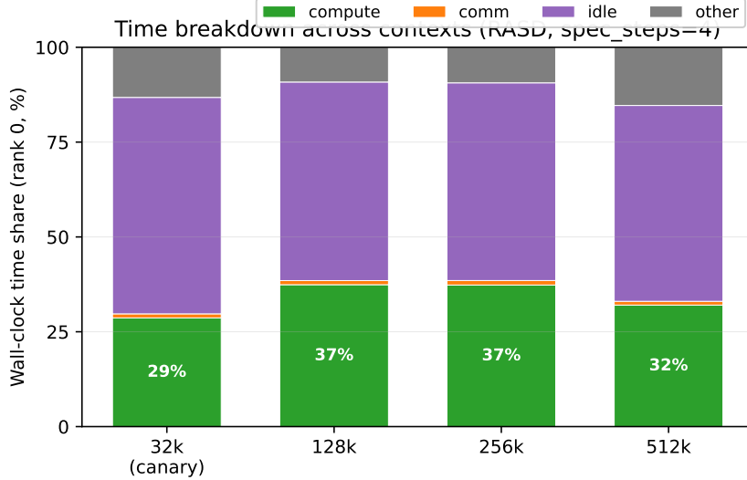
Figure 4: Stacked-bar time breakdown for rank-0 across contexts. “Compute” is real GPU work (matmul, attention, layernorm, etc.); “comm” is NCCL + ring-exchange collectives; “idle” is wall not attributable to GPU events (rank-0 waiting on other ranks); “other” is allocator and kernel-launch overhead. Annotated value is the compute share.
