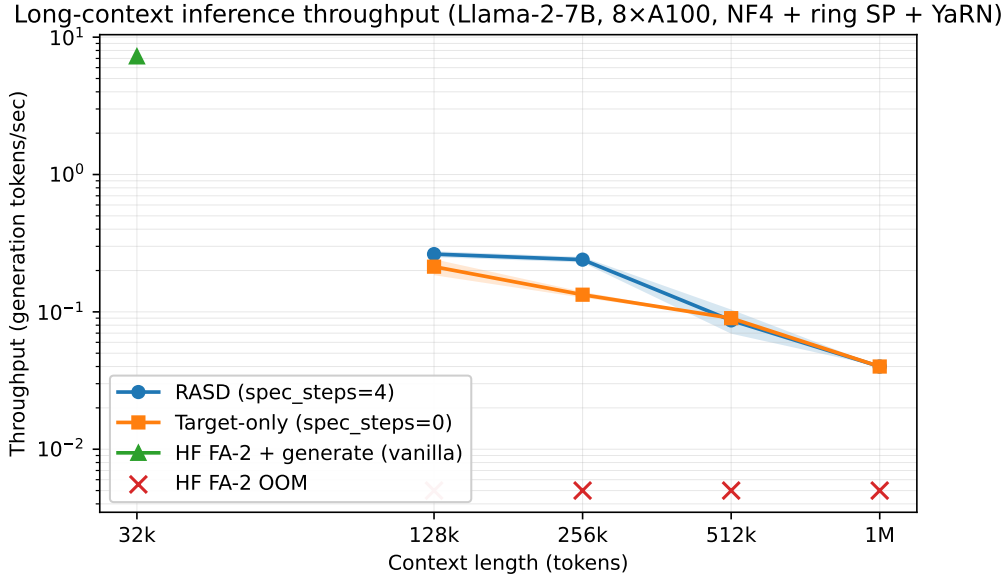
Figure 3: Throughput vs. context length. RASD spec mode (●) and matched target-only baseline (■) at 4 contexts \times 3 seeds; vanilla HF FA-2 generate() (▲) at 32k only, OOM markers (×) for \geq 128k . Bands are 95% bootstrap CI over 3 seeds. Both axes log scale.
