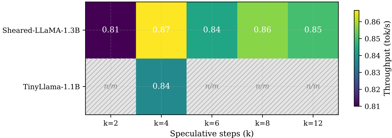
M3 ablation: Throughput (tok/s) (R6.5, ctx=64k, 8×A100-SXM4-40GB)
