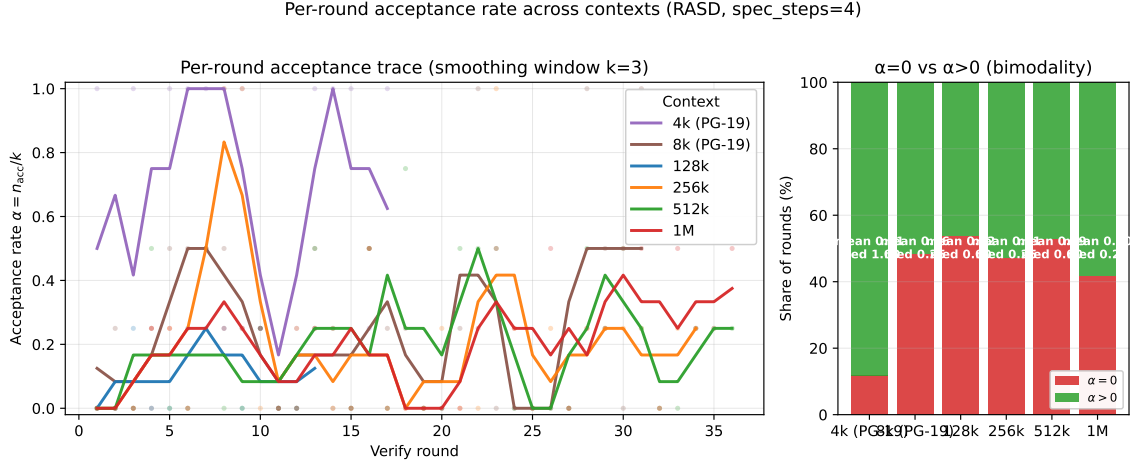
Figure 6: (Left) per-round acceptance \alpha = n_{acc}/k for RASD across six contexts (4k and 8k with PG-19 prompts, 128k–1M with synthetic prompts), smoothed by a 3-round rolling mean. Raw points faded behind. (Right) Bimodality view: share of rounds at \alpha = 0 vs \alpha > 0 per context, annotated with mean and median \alpha .
