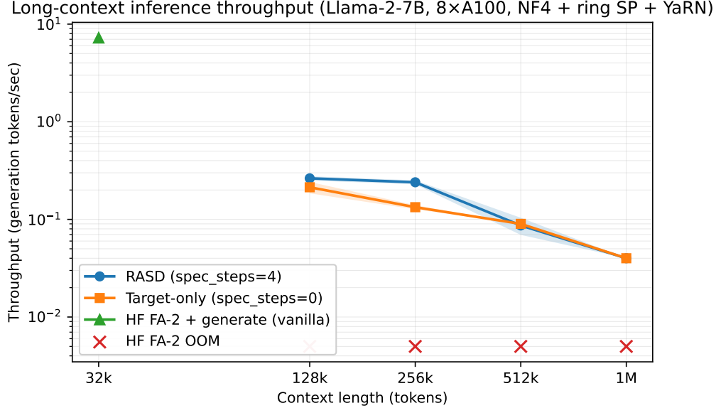
Figure 4: Throughput vs. context length. RASD spec mode (●) and matched target-only baseline (■) at 4 contexts \times 3 seeds; vanilla HF FA-2 generate() (▲) at 32k only, OOM markers (×) for \geq 128 k. Bands are 95% bootstrap CI over 3 seeds. Both axes log scale.
