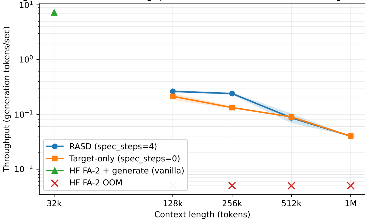
Long-context inference throughput (Llama-2-7B, 8×A100, NF4 + ring SP + YaRN)
