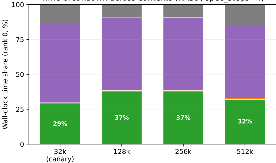
Time breakdown across contexts (RASD, spec_steps=4)
