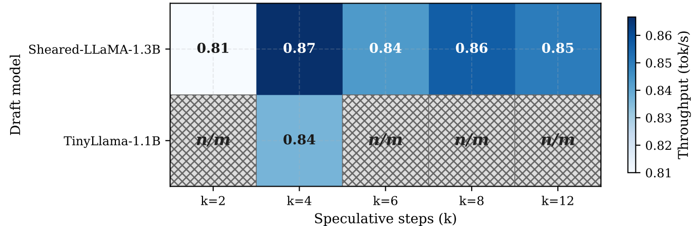
M3 ablation: Throughput (tok/s) (ctx=64k, 8×A100-SXM4-40GB)
