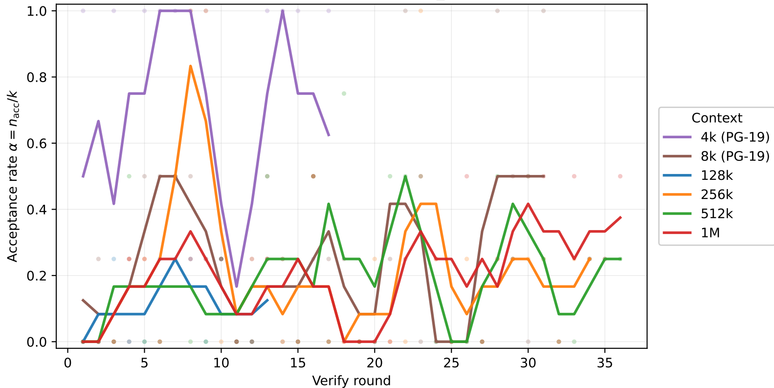
Per-round acceptance trace across contexts (RASD, spec_steps=4, smoothing window k=3)
