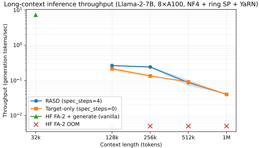
Figure 1: Throughput vs. context length. RASD spec mode (●) and matched target-only baseline (■) at 4 contexts \times 3 seeds; vanilla HF FA-2 generate() (▲) at 32k only, OOM markers (×) for \geq 128 k. Bands are 95% bootstrap CI over 3 seeds. Both axes log scale.
