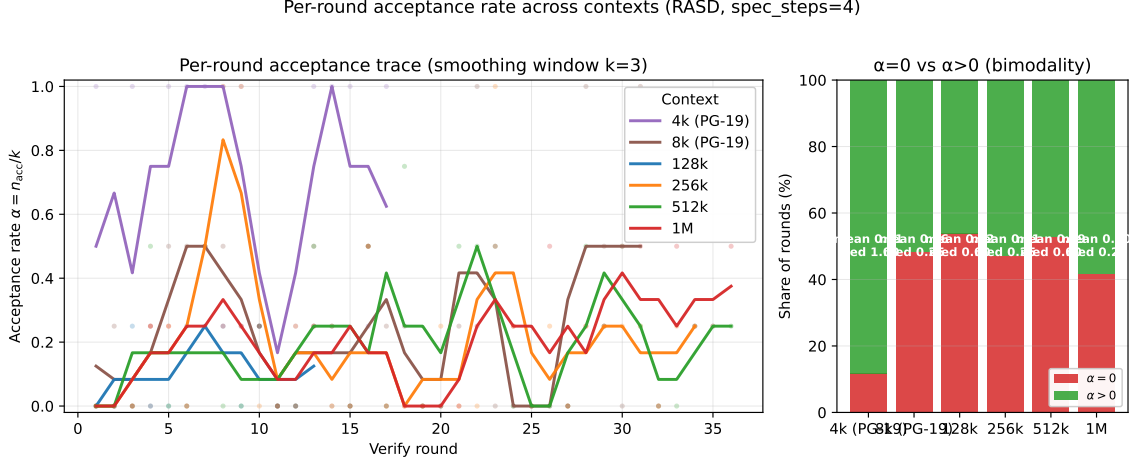
Figure 3: (Left) per-round acceptance \alpha = n_{acc}/k for RASD across six contexts (4k and 8k with PG-19 prompts, 128k–1M with synthetic prompts), smoothed by a 3-round rolling mean. Raw points faded behind. (Right) Bimodality view: share of rounds at \alpha = 0 vs \alpha > 0 per context, annotated with mean and median \alpha .
