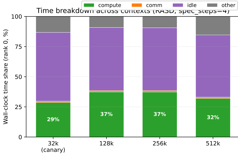
Figure 2: Stacked-bar time breakdown for rank-0 across contexts. “Compute” is real GPU work (matmul, attention, layernorm, etc.); “comm” is NCCL + ring-exchange collectives; “idle” is wall not attributable to GPU events (rank-0 waiting on other ranks); “other” is allocator and kernel-launch overhead. Annotated value is the compute share.
