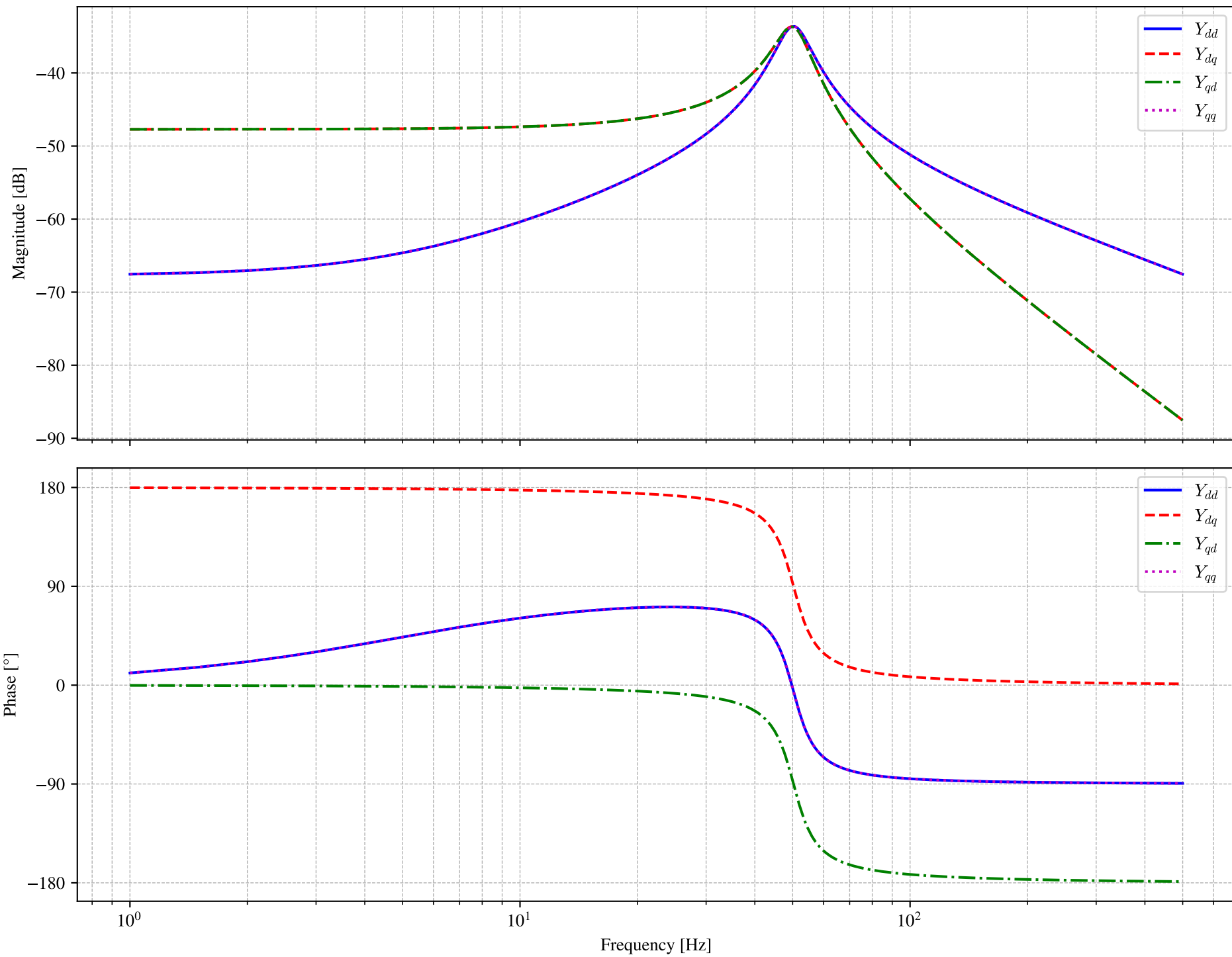
Bode Plot of Admittance: Y_Grid
