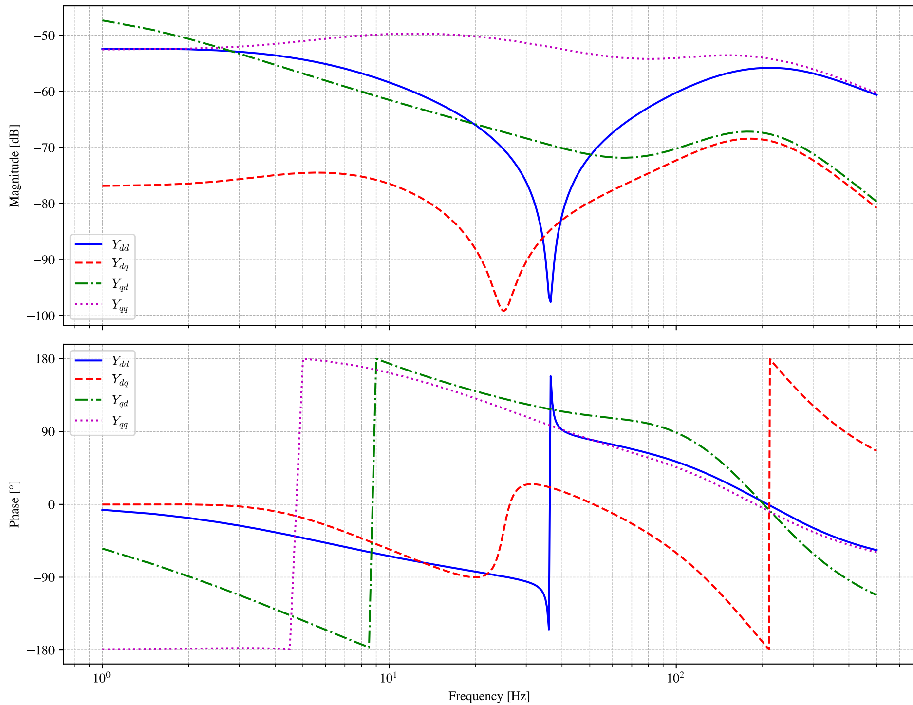
Bode Plot of Admittance: Y_{VSC}
