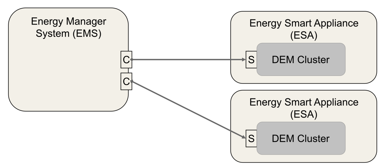
Figure 19. Example of the how an EMS is a client of multiple ESAs Device Energy Management clusters.
