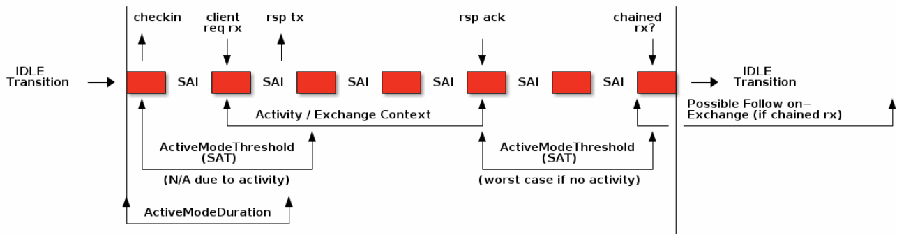
Figure 79. ICD Active Mode Behavior Diagram
