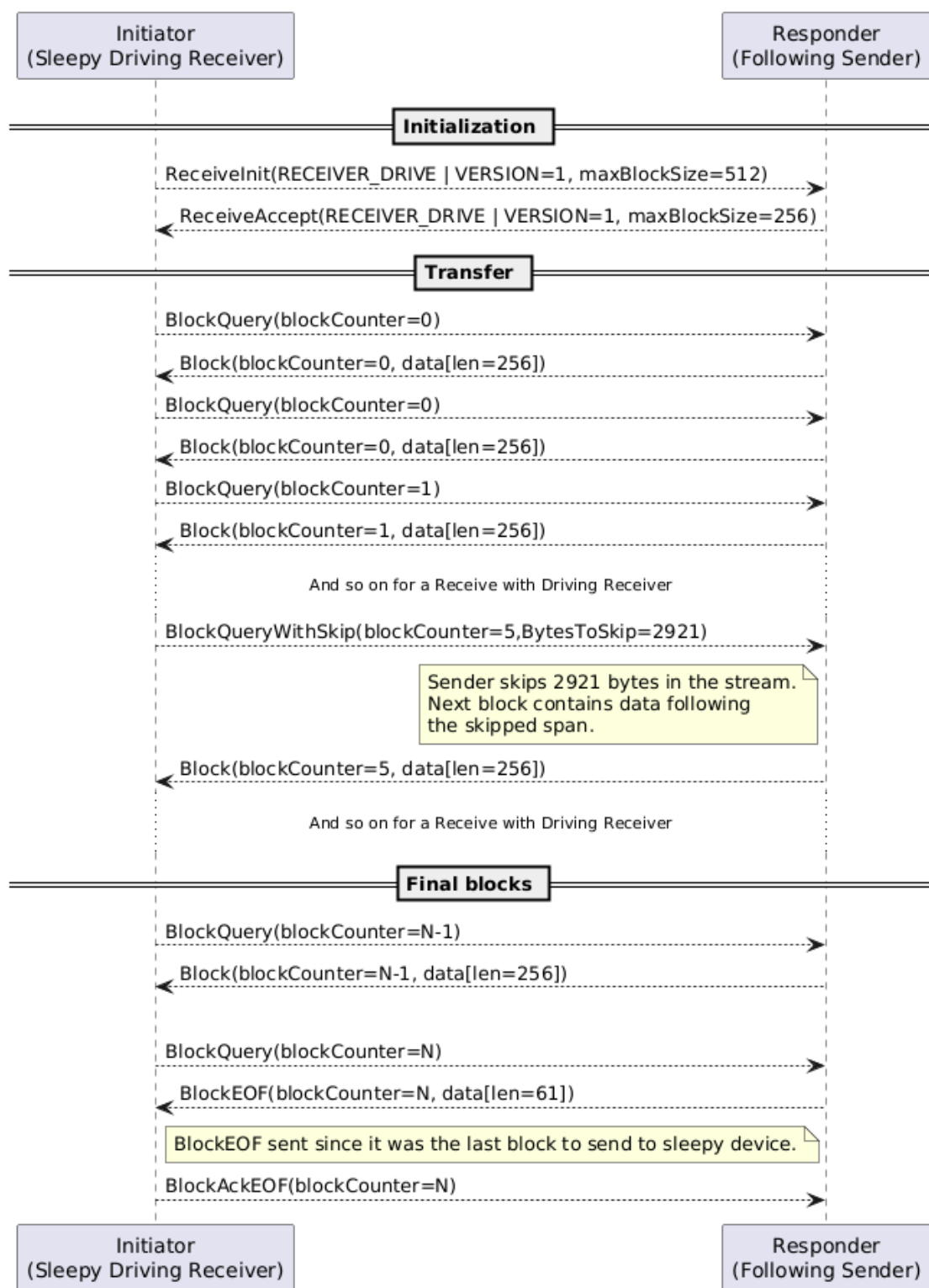
Figure 102. Synchronous file receiving by device acting as driving Receiver, including BlockQueryWithSkip
