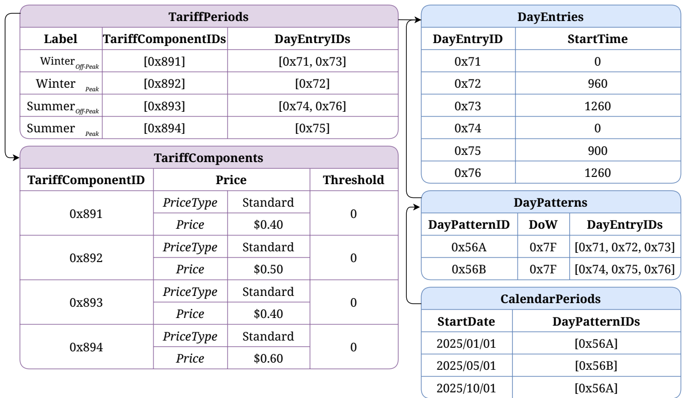
Figure 26. Example of a seasonal time-of-use rate commodity tariff
