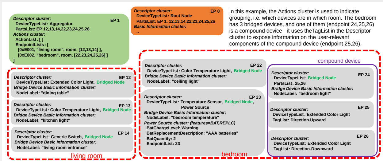
Figure 10. use of NodeLabel and TagList for disambiguation
