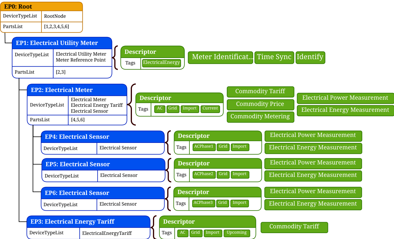
Figure 31. Example of a phased Electrical Utility Meter
