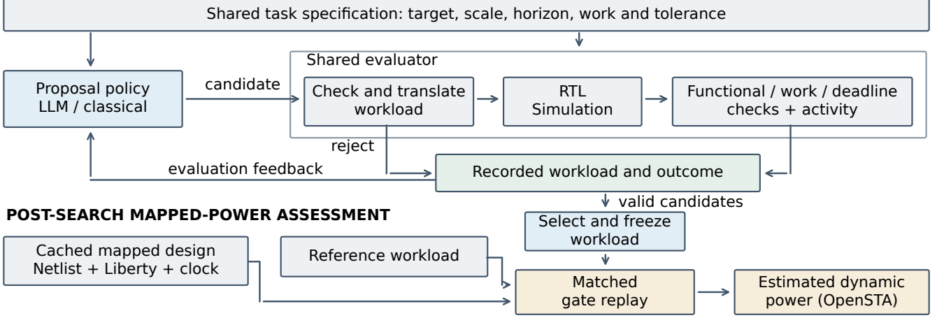
Fig. 1. Simulation feedback guides workload proposals. After search, the selected workload and a separately constructed reference are replayed on the synthesized design under the same conditions. Estimated power assesses the result but does not guide search.
