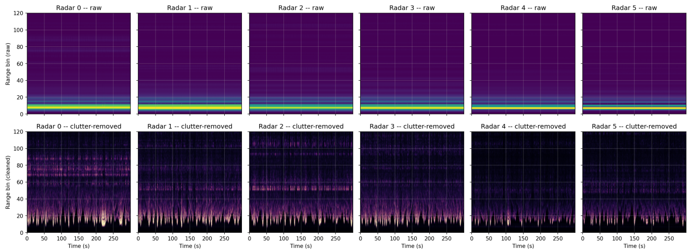
Effect of running-mean clutter removal ( W=50 frames = 2.0 s)
