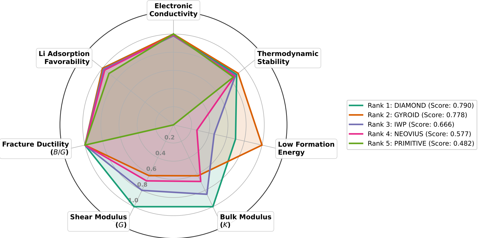
Figure 10: Holistic 7-Axis Performance Radar Map for Graphene TPMS Topologies across Core Functional Anode Properties
