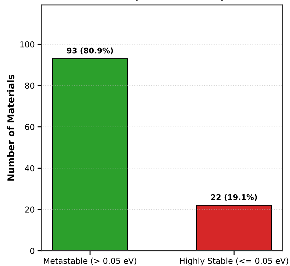
(b) Thermodynamic Stability ( E_{\text{hull}} )
