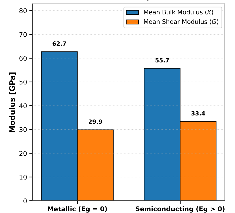
(c) Mean Elastic Moduli by Electronic Class
