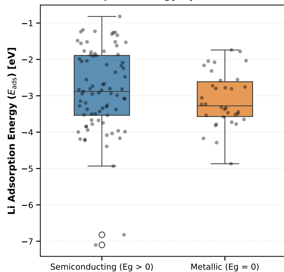
(d) Li Adsorption Energy by Electronic Class
