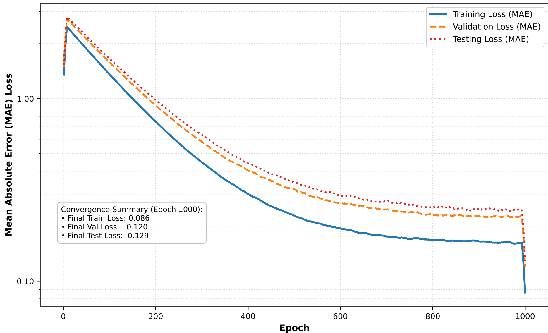
Figure 4: CGCNN Multi-Property Training Convergence (1,000 Epochs)
