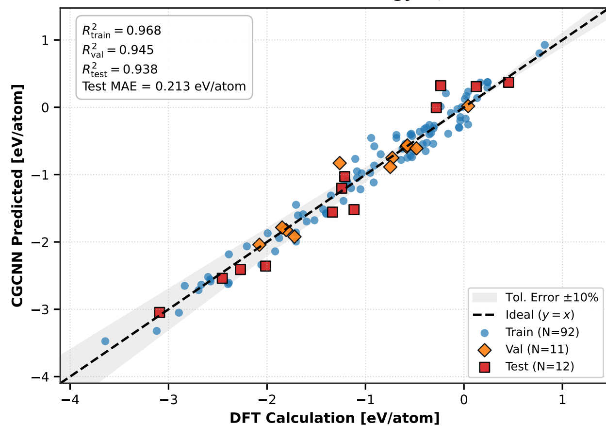
(b) Formation Energy ( E_f )
