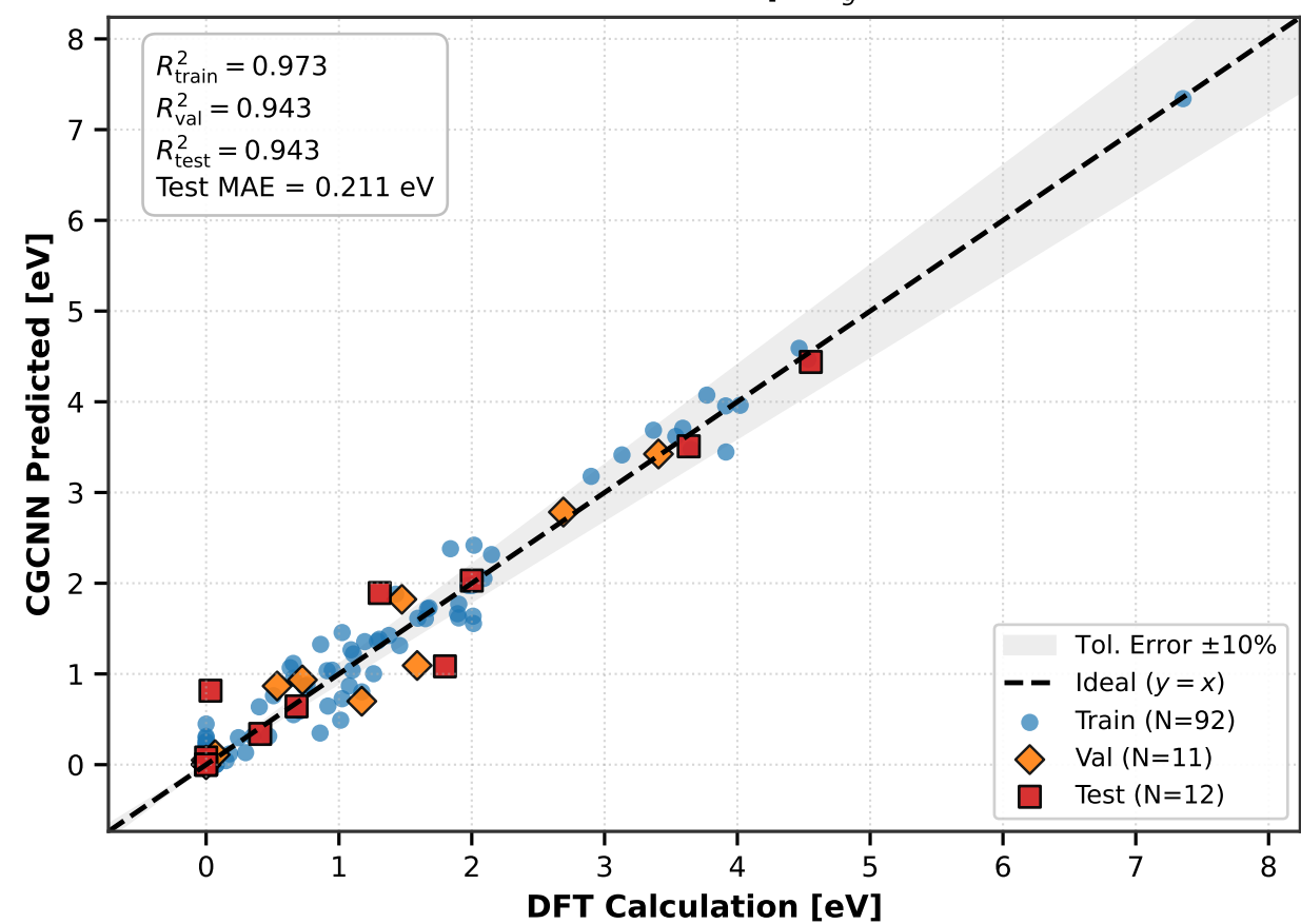
(a) Band Gap ( E_g )
