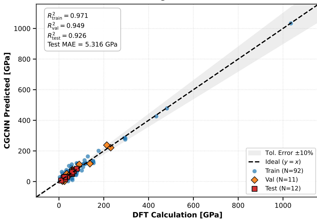
(f) Young's Modulus ( E )
