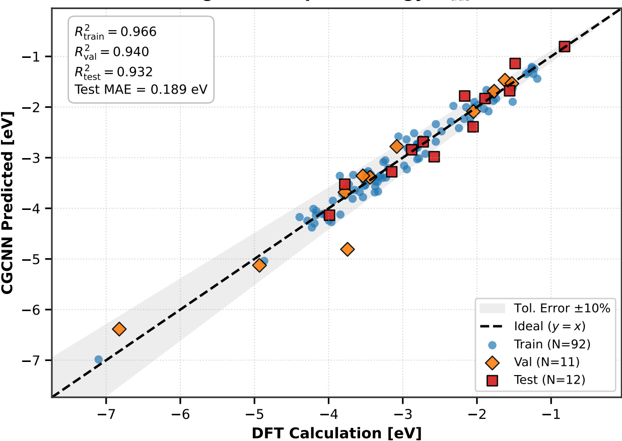
(g) Li Adsorption Energy ( E_{\text{ads}} )
