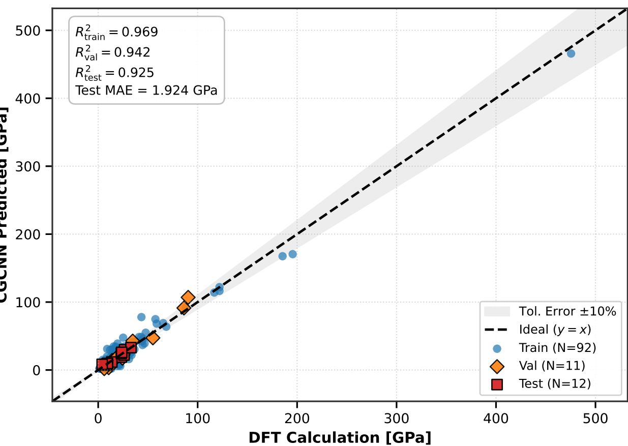
(e) Shear Modulus ( G )
