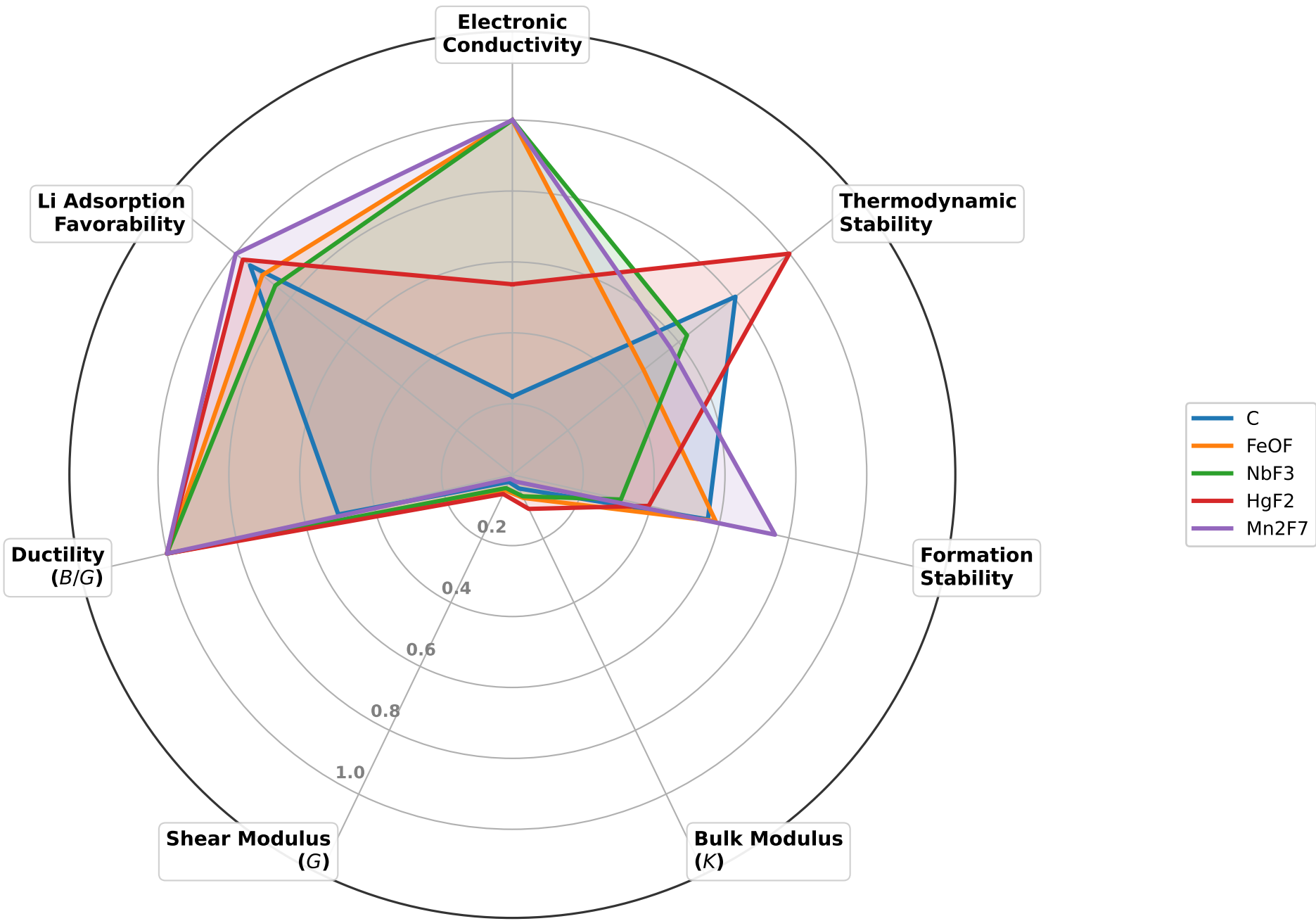
Figure 8: Holistic 7-Axis Performance Radar Map for Top 5 Host Anodes
