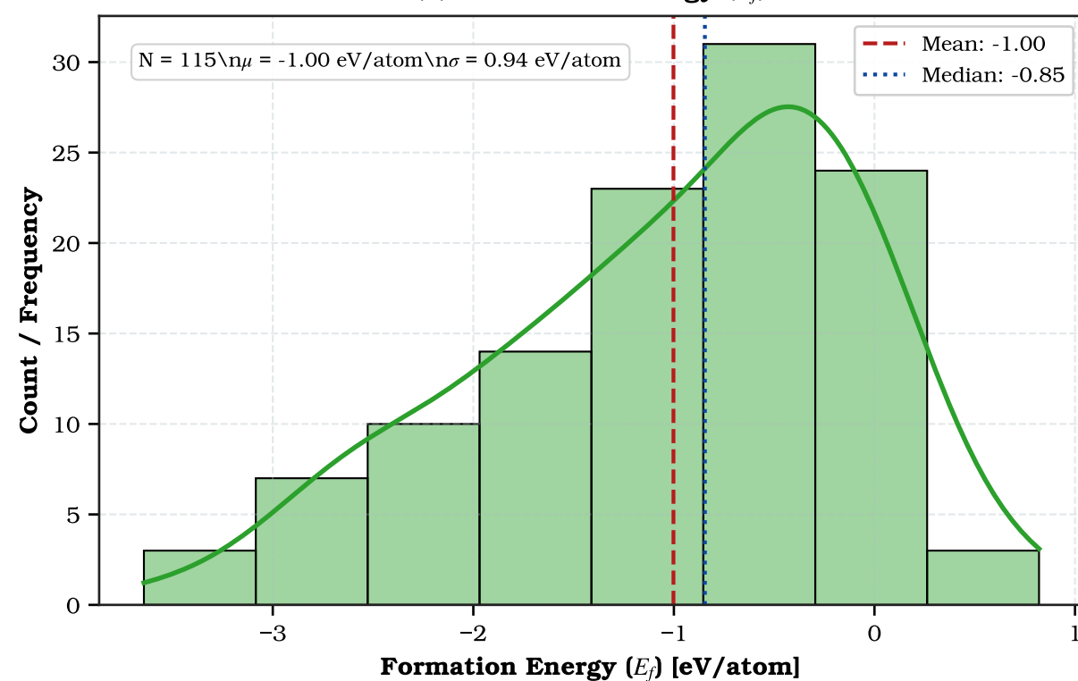
(b) Formation Energy ( E_f )
