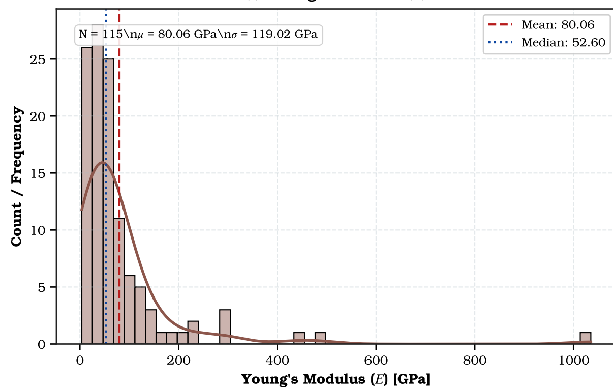
(f) Young's Modulus ( E )
