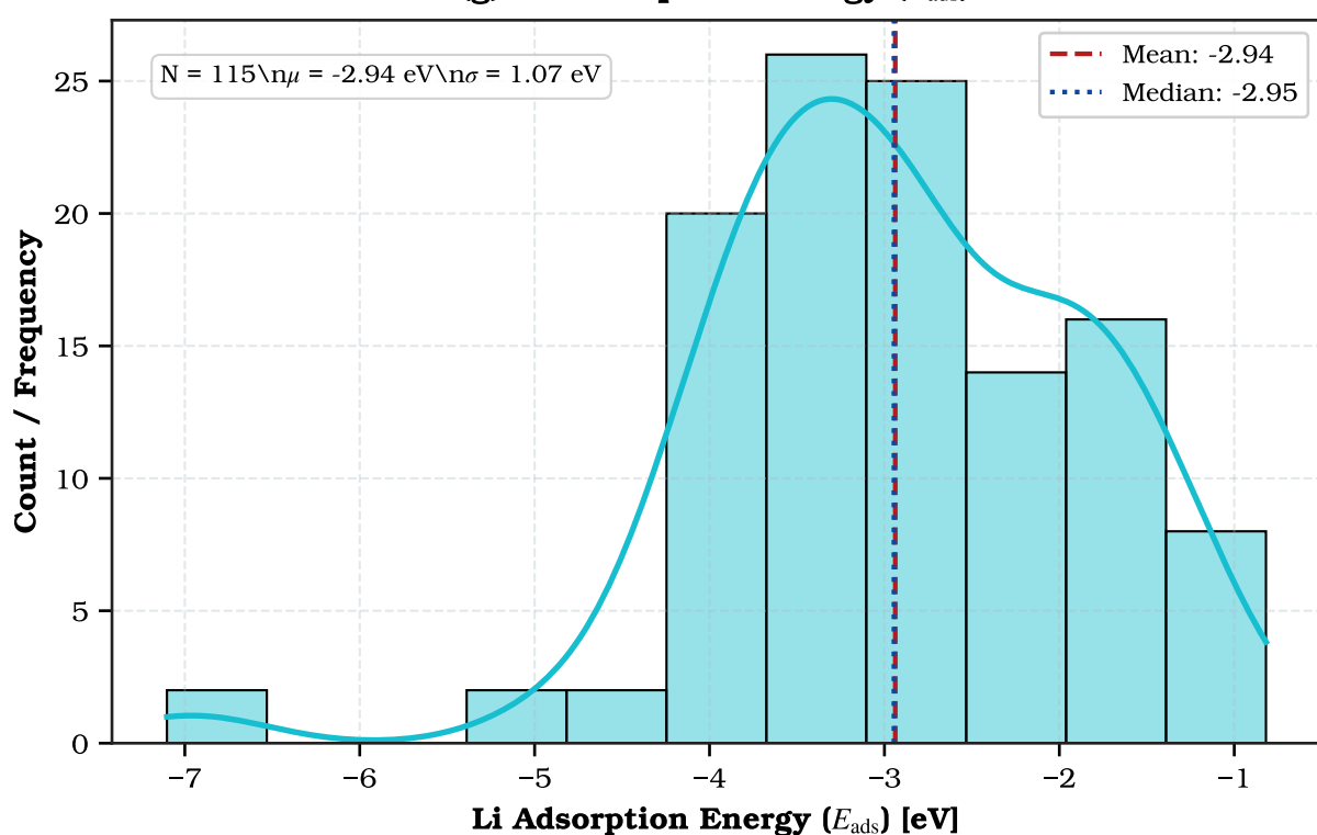
(g) Li Adsorption Energy ( E_{\text{ads}} )
