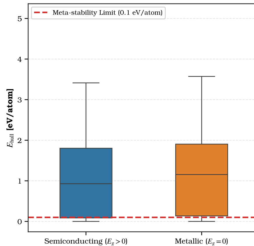
(b) Thermodynamic Stability ( E_{\text{hull}} )
