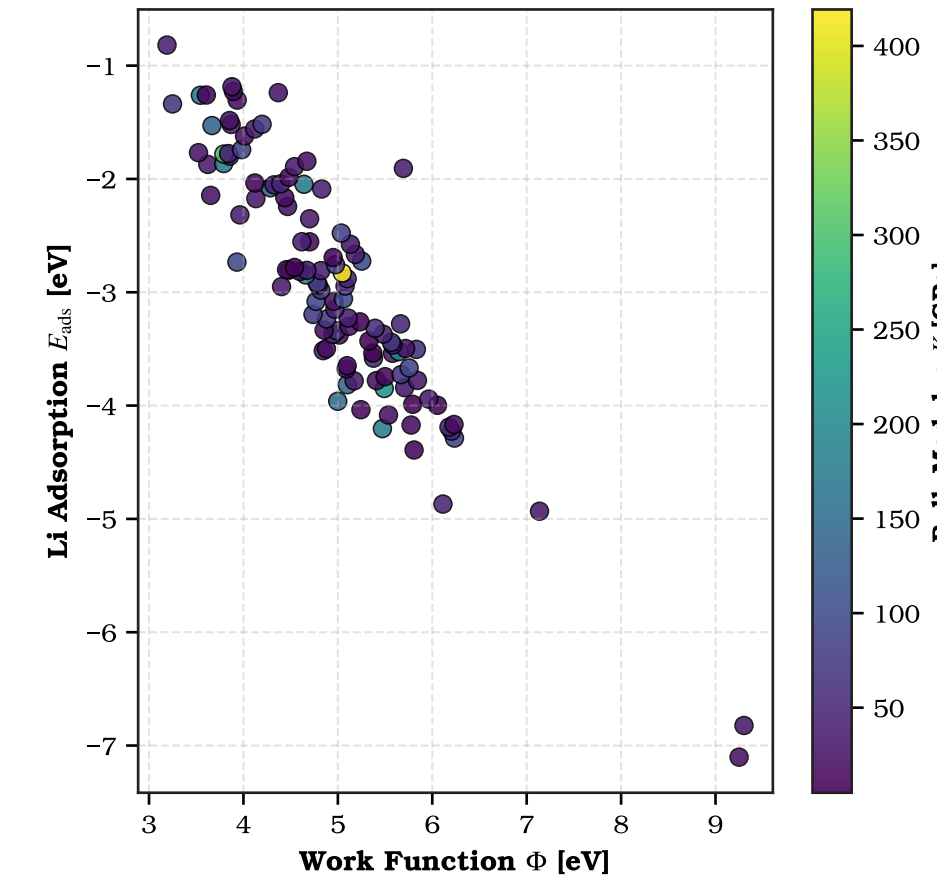
(f) Work Function vs Li Adsorption Landscape
