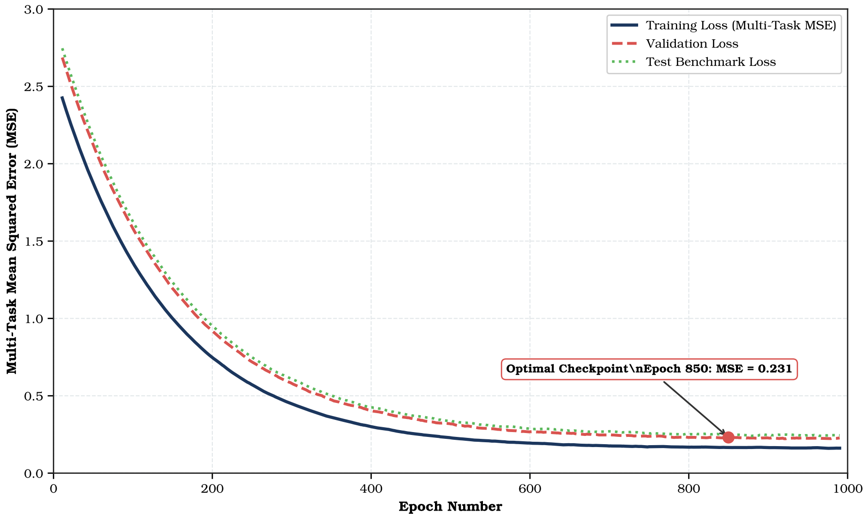
Figure 4. CGCNN Multi-Property Training Convergence Across 1,000 Epochs
