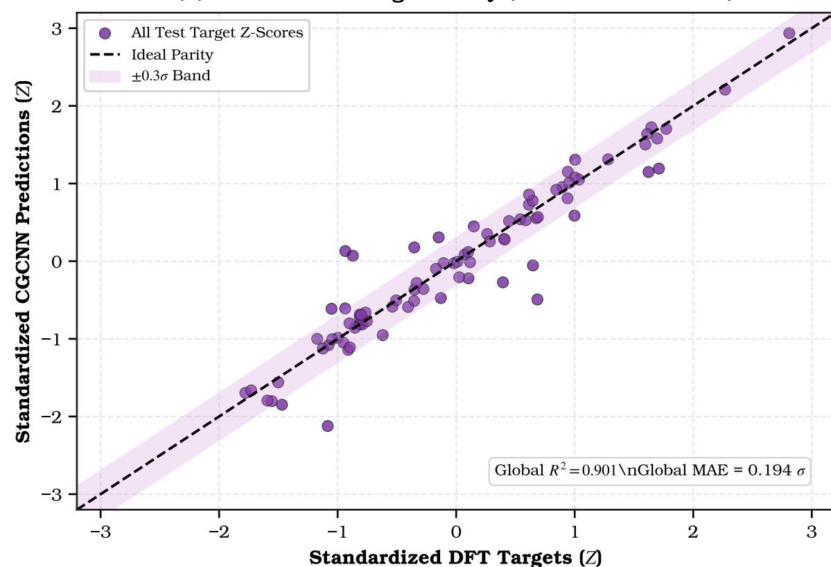
(h) Global Multi-Target Parity (Z-Score Normalized)
