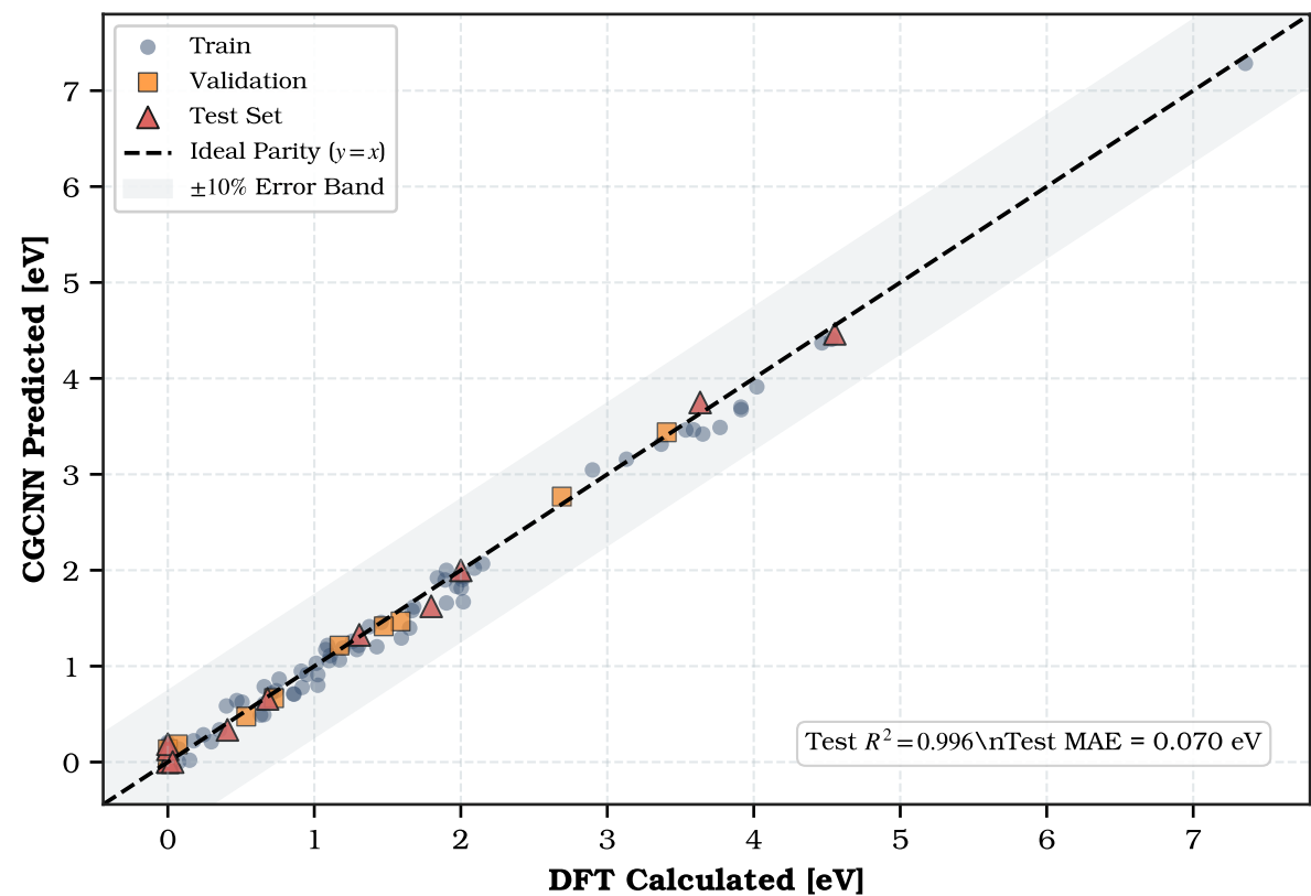
(a) Band Gap ( E_g )
