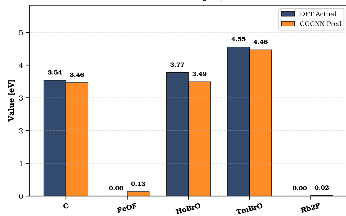
(a) Band Gap ( E_g )
