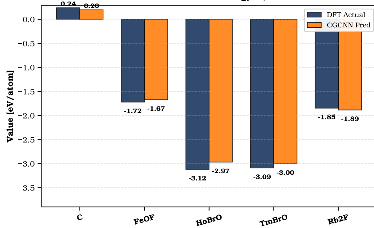
(b) Formation Energy ( E_f )
