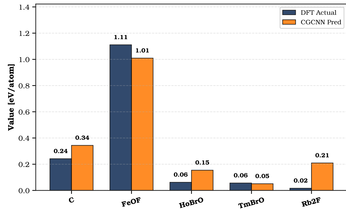
(c) Energy Above Hull ( E_{\text{hull}} )
