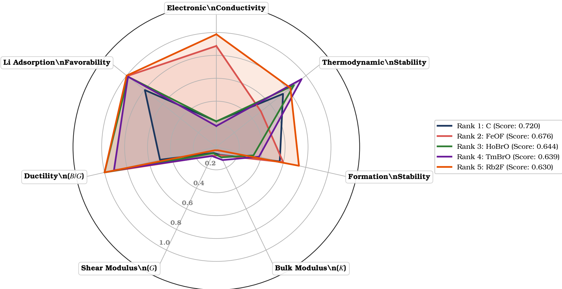
Figure 8. Holistic 7-Axis Performance Radar Map for Top 5 Host Anodes
