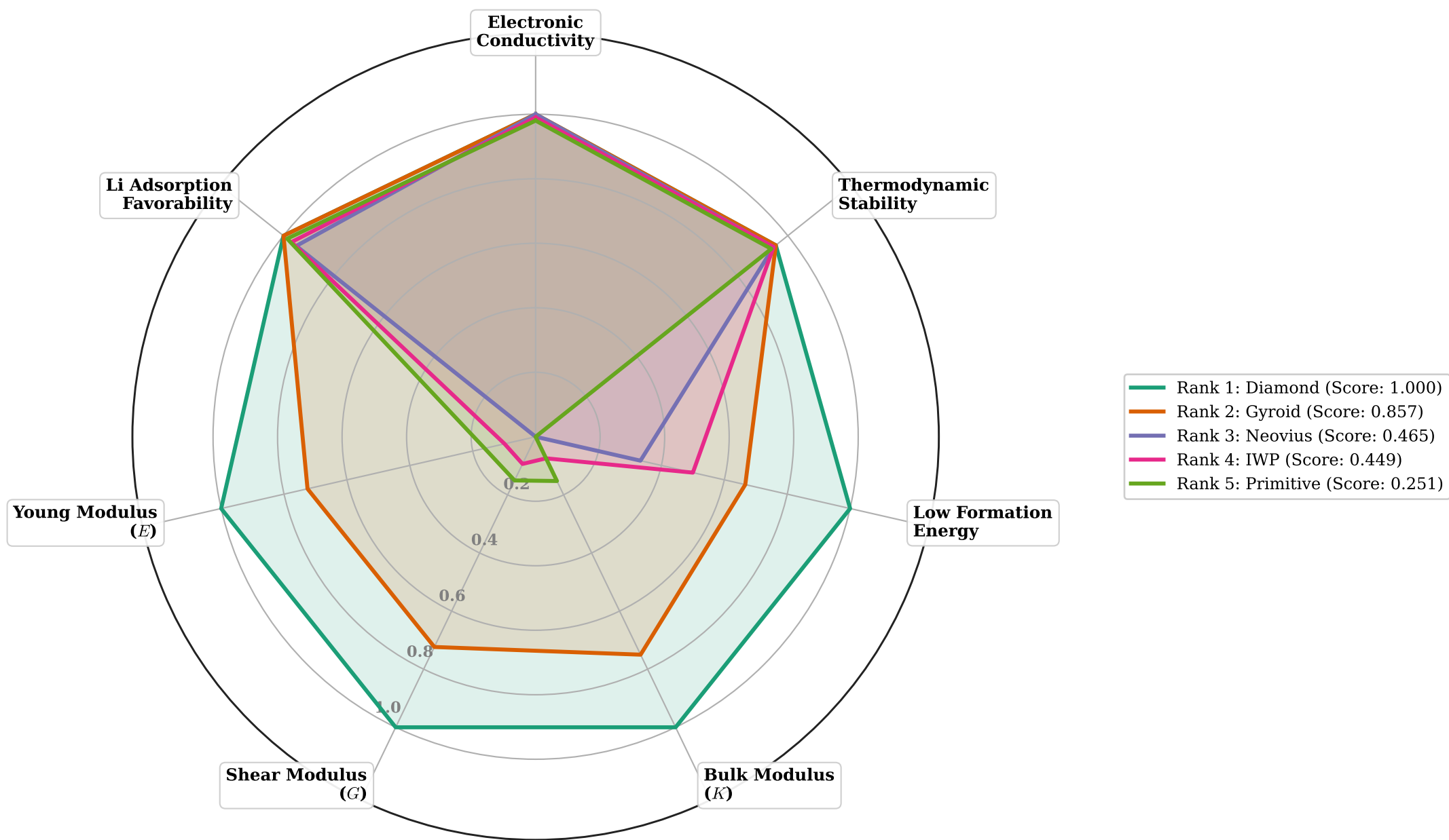
Figure 10. Holistic 7-Axis Performance Radar Map for Graphene TPMS Topologies
