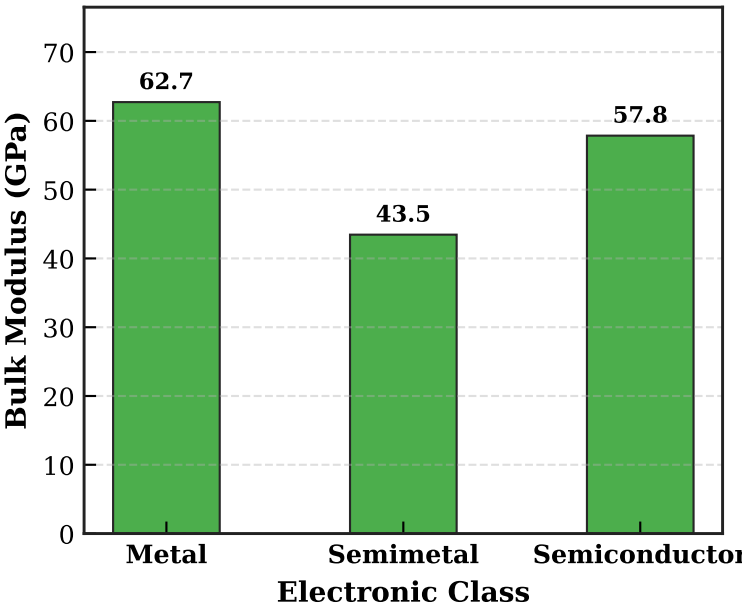
(c) Mean Bulk Modulus (GPa)
