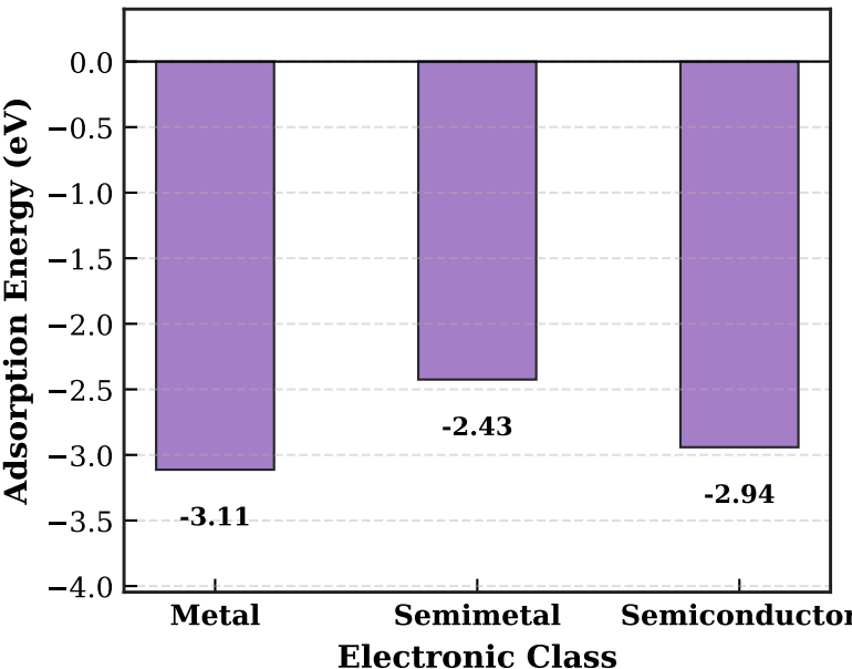
(f) Mean Li Adsorption Energy ( E_{\text{ads}} , eV)
