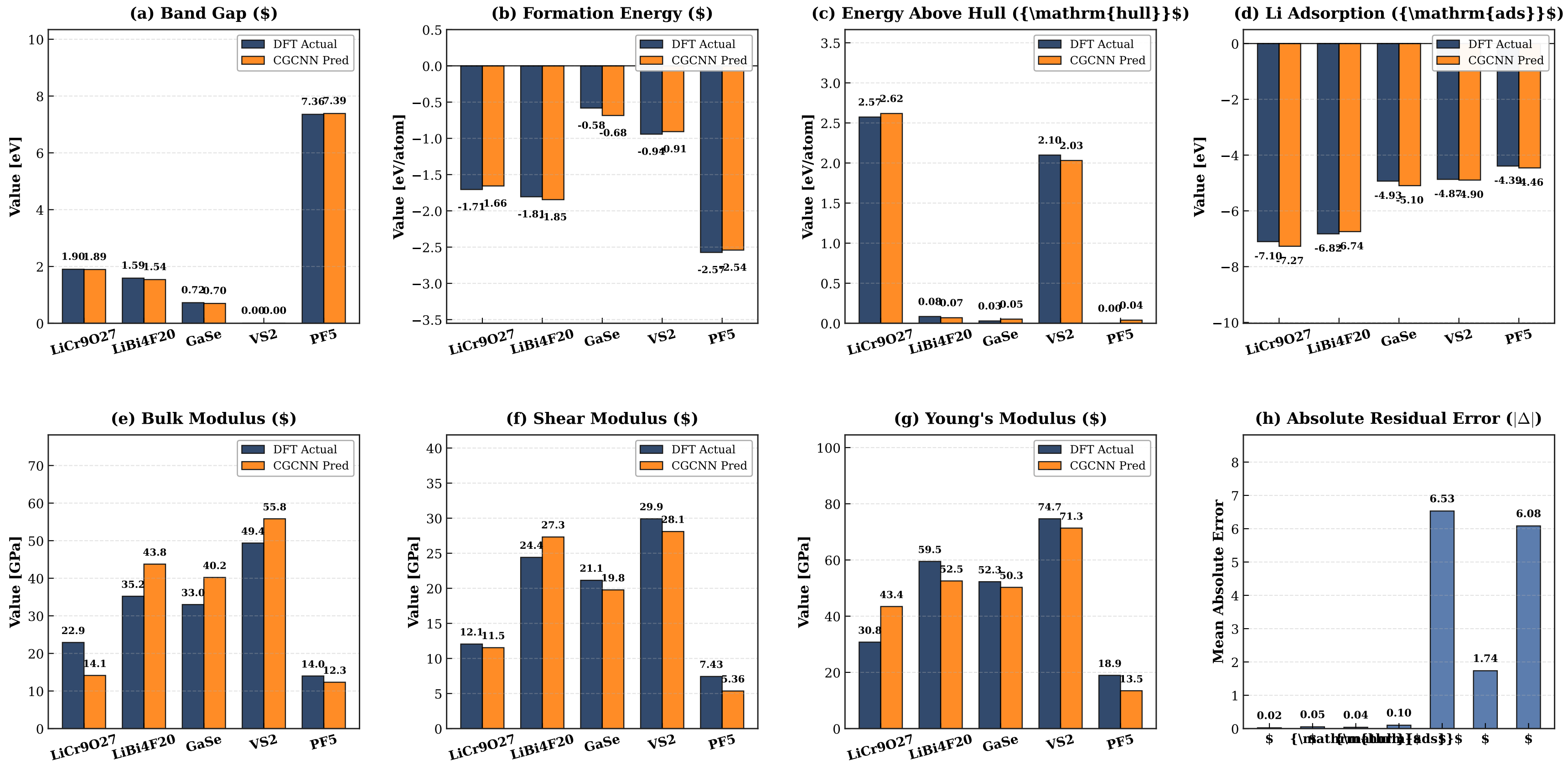
Figure 6. DFT Actual vs CGCNN Predicted Properties for First 5 Raw Dataset Materials
