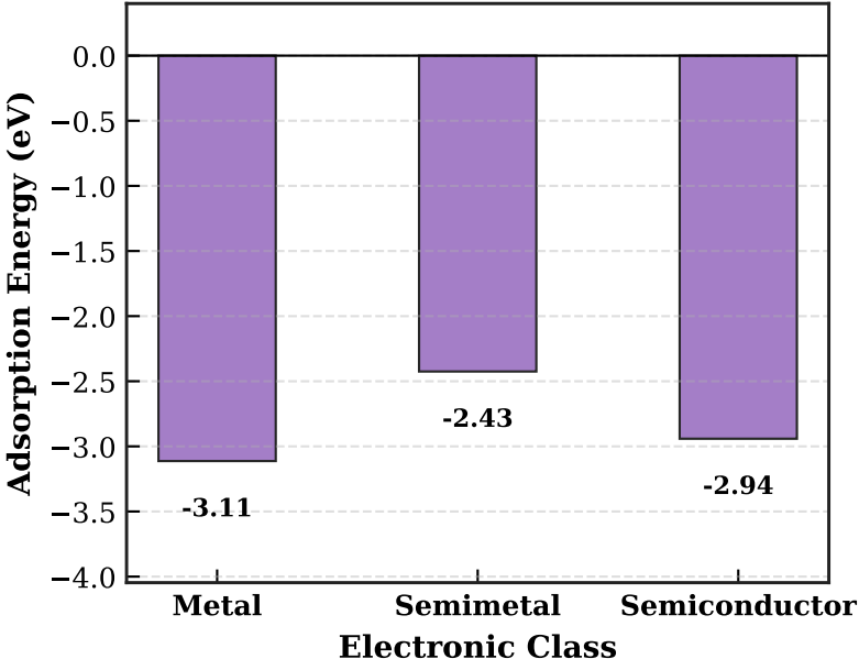
(f) Mean Li Adsorption Energy ( E_{\text{ads}} , eV)
