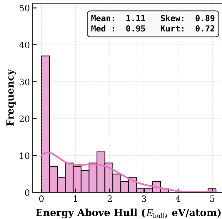
(c) Energy Above Hull
