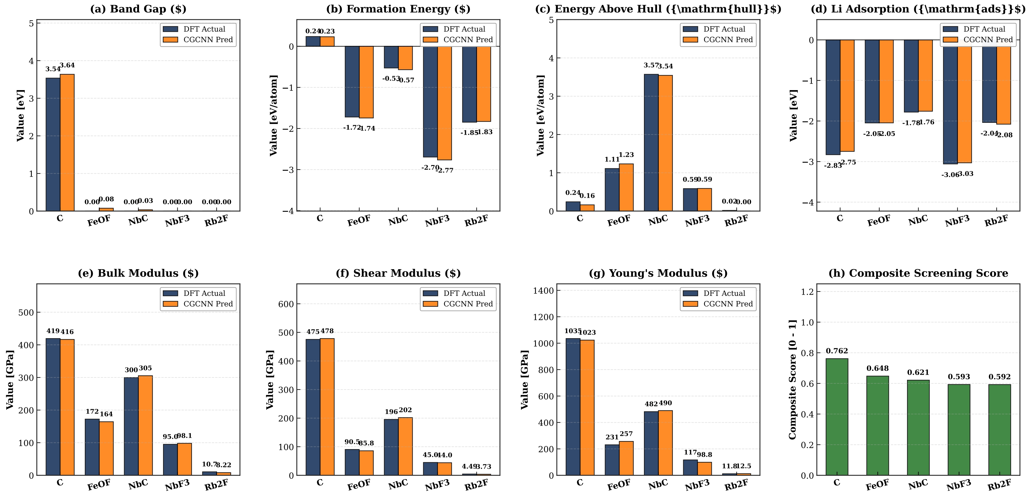
Figure 7. DFT Actual vs CGCNN Predicted Properties for Top 5 Candidate Anode Materials
