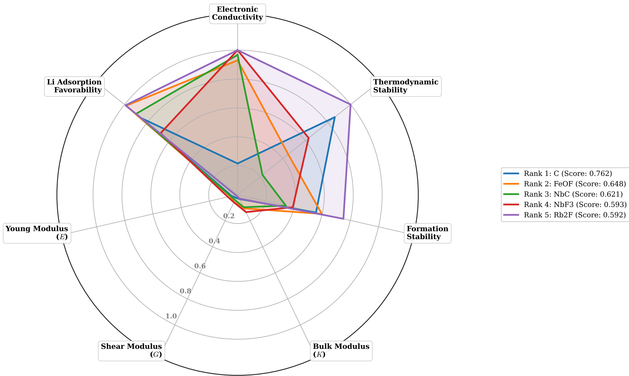
Figure 8. Holistic 7-Axis Performance Radar Map for Top 5 Candidate Anode Materials
