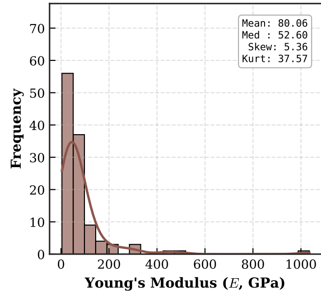
(f) Young's Modulus
