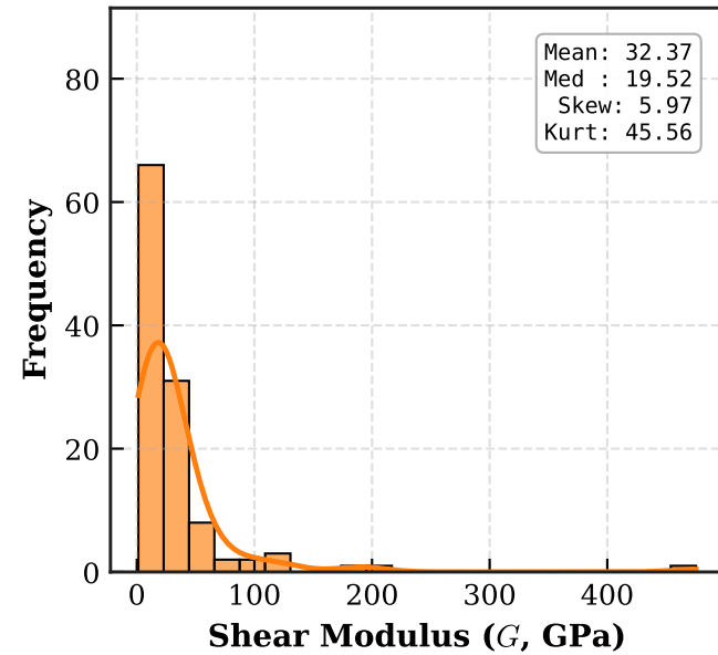
(e) Shear Modulus
